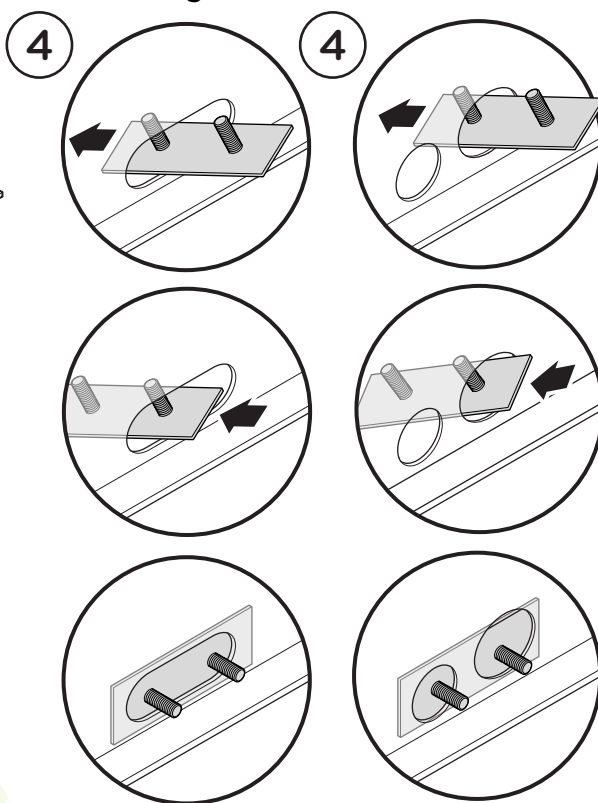
Front Bracket Oblong Hole
