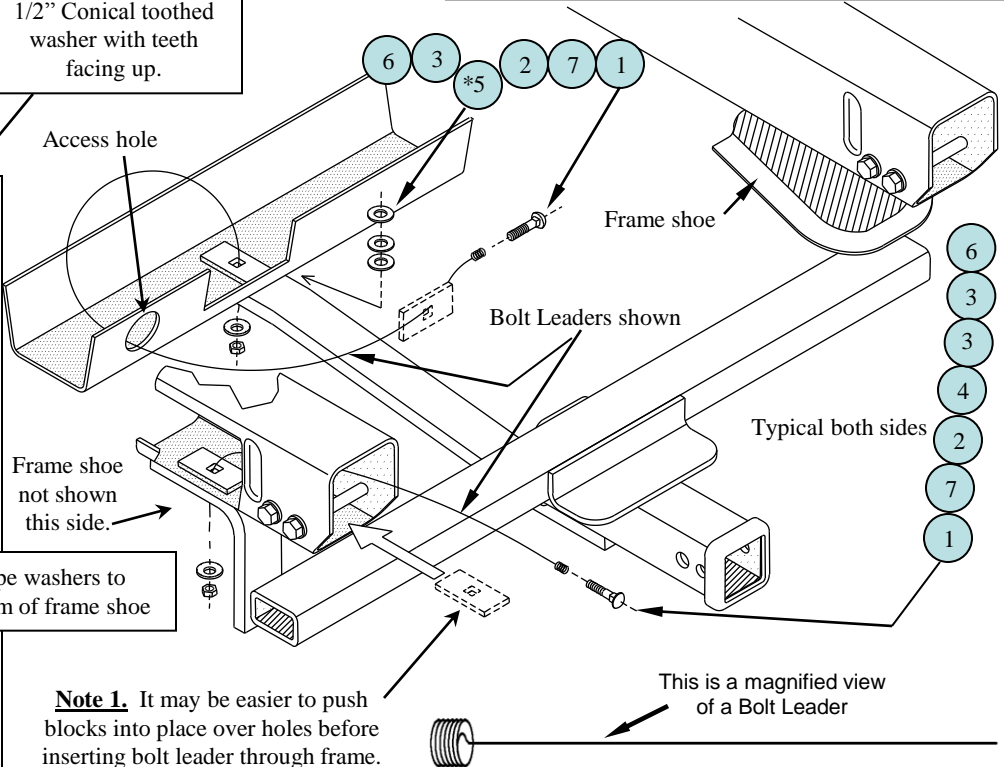
Frame shoe Detail A
