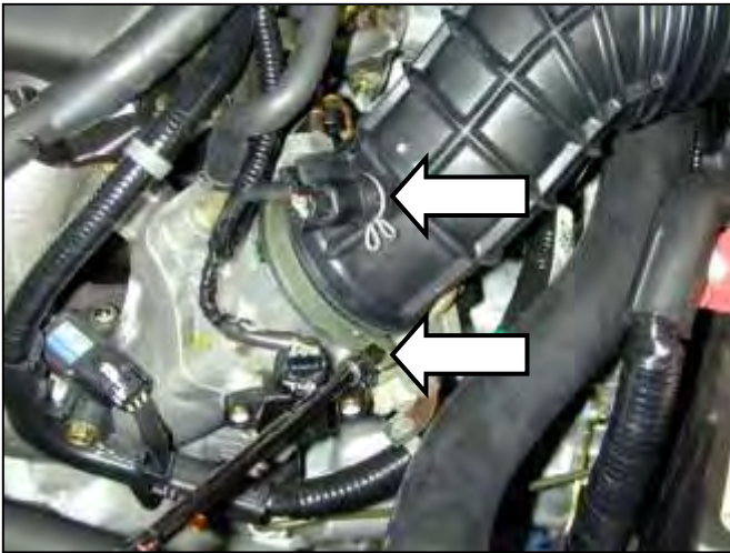
a. Loosen the clamp around the throttle body. Pull the intake air temperature (IAT) sensor out of the intake tube by loosening the spring loaded clamp.
