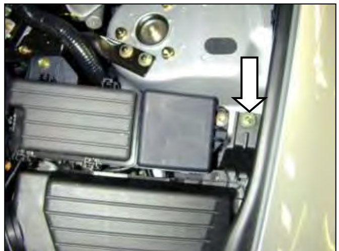
d. Remove the other airbox mounting bolt shown in the picture.
