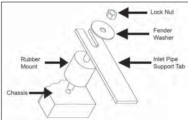
h. Proper installation of the rubber mount assembly.
