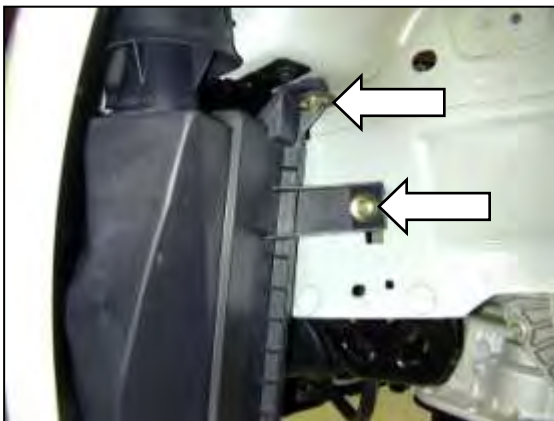
i. Remove the two screws near the upper rear section of the lower airbox.
