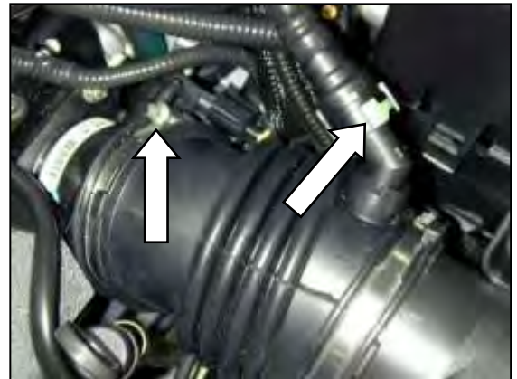
b. Release the fitting on the inlet pipe nipple and loosen the hose clamp at the throttle body.
