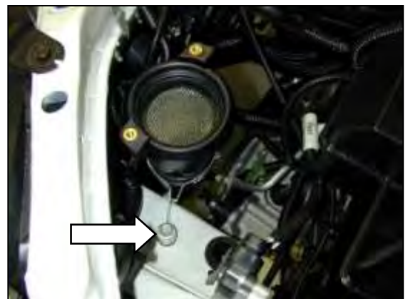
d. Remove the upper airbox and the bolt in the frame rail. Release the metal clamp from the Mass Air Flow (MAF) sensor housing.
