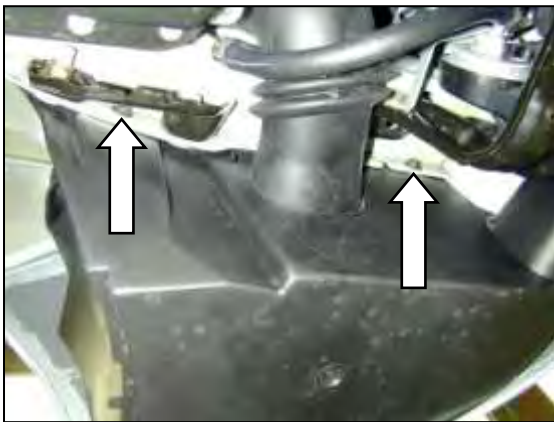
g. From underneath the vehicle, remove the two screws that secure the splash shield.
