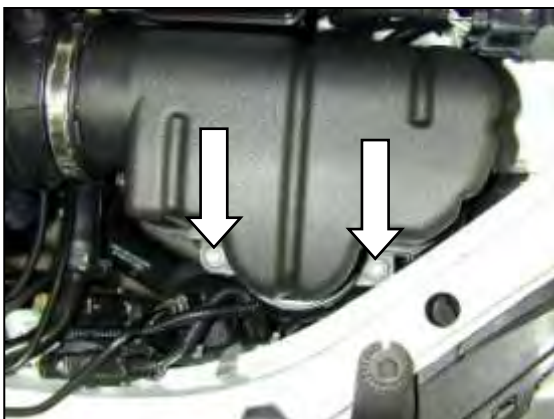
c. Loosen the two bolts that secure the upper airbox.
