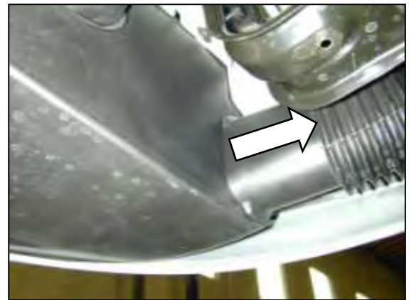
h. Pull the air snorkel from the splash shield and remove the splash shield.
