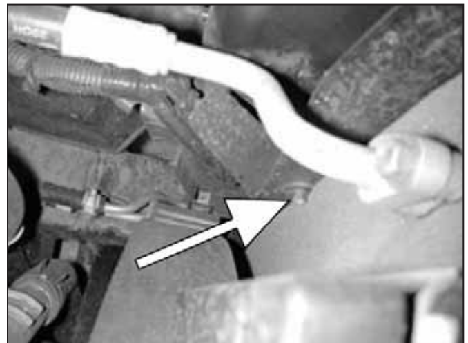
j. The washer bottle must now be removed. Remove the small screw next to the left side of the radiator.
