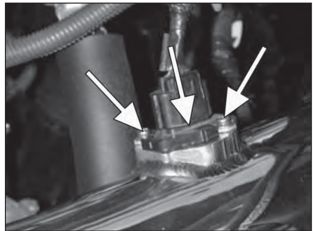
q. Install the factory MAFS into the inlet pipe utilizing the stock screws. Plug in the MAFS. Reinstall the engine cover.
