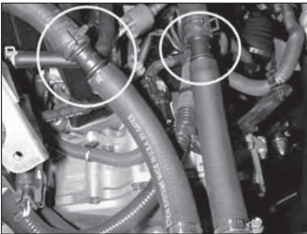
p. Connect the factory breather hoses to the open ends of the hoses with the supplied nylon barbed fittings.
