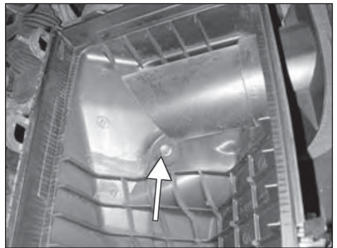
h. Remove the upper airbox and filter. Loosen the bolt on the bottom of the box.
