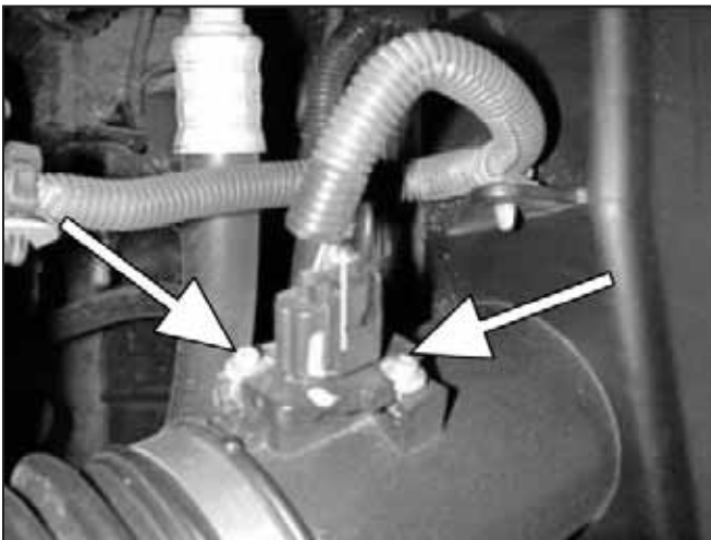
c. Unplug the Mass Air Flow Sensor (MAFS) and pinch the rivet to release the wiring harness. Release the two screws retaining the MAFS. Gently remove the MAFS and place aside. Handle the MAF sensor with care to avoid damaging it.
