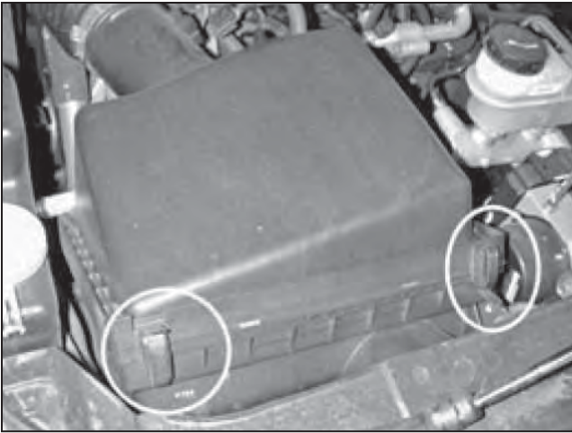
e. Release the two clips on the side of the airbox.
