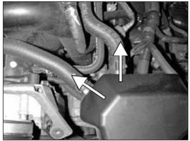
d. Pinch the two hose clamps and pull the breather hoses from the airbox.
