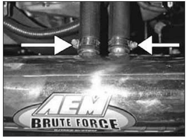
o. Attach the two supplied breather hoses to the inlet pipe with the supplied size 10 hose clamps.
