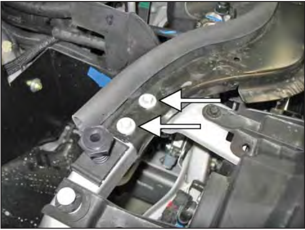
g. Insert the heat shield tab underneath the hood latch support bracket. Secure with factory hardware.
