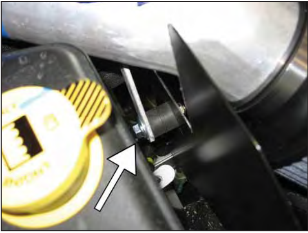
m. Secure the inlet pipe to the rubber mount with M8 washer and nut.
