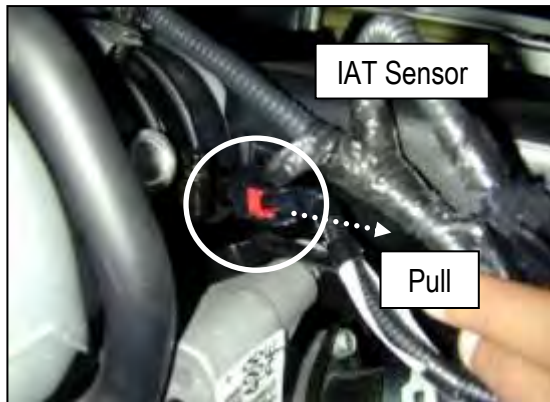
c. Disconnect the Inlet Air Temperature (IAT) sensor by first pulling the tab away from the sensor. Then push in on the clip to disconnect. Remove the sensor from the inlet tube by gently pulling away from the tube.
