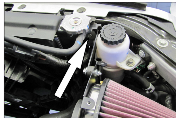
19. Install the heat shield bracket assembly onto the heat shield and radiator mount as shown. Secure the bracket with the factory bolt from step number 9 and the hardware provided.
