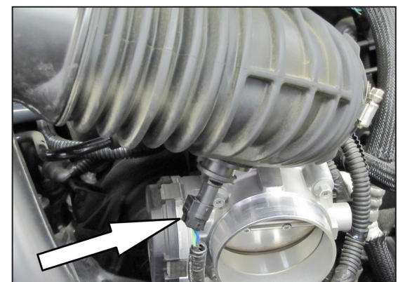
6. Lift up the intake tube and then disconnect the inlet air temperature electrical connection. Then remove the intake tube from the vehicle.
