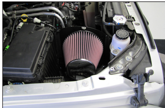
17. Install the K&N® air filter onto the filter adapter and secure with the provided hose clamp.
