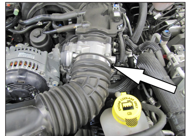
5. Loosen the hose clamp securing the factory intake tube to the throttle body.
