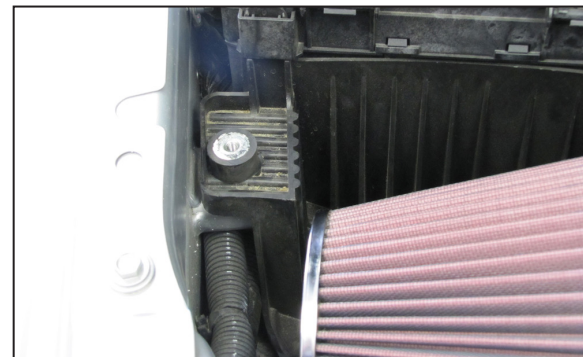
20. Install the rubber mounted stud into the into the air box mounting plate bolt location as shown.
