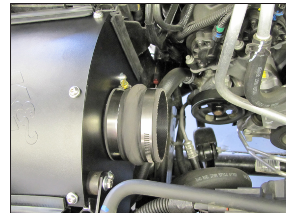
23. Install the provided hump hose (08699) onto the filter adapter and secure with the provided hose clamp.
