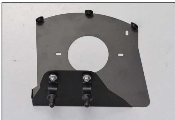
12. Install the two heat shield bracket assemblies onto the heat shield as shown.
