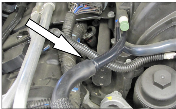
7. Disconnect the crank case vent hose from the crank case vent tube.
