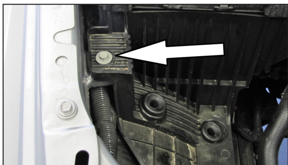
9. Remove the bolt shown that secures the air box mount bracket to the inner fender.
