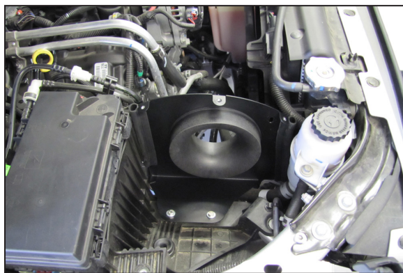
16. Install the heat shield assembly into position so the mounting studs are in the air box mounting grommets.
