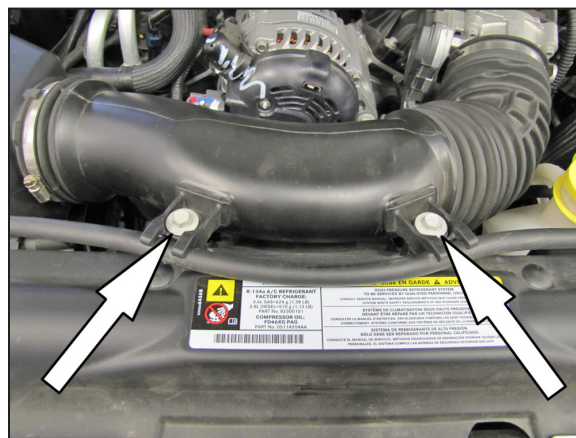
3. Remove the two bolts which secure the factory intake tube to the fan shroud.
