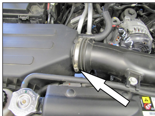
4. Loosen the hose clamp securing the factory intake tube to the air filter housing.
