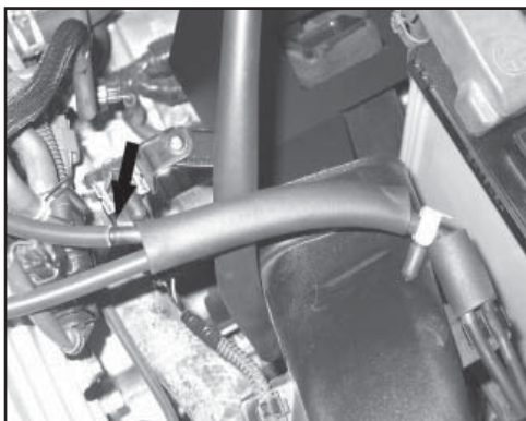
31. Connect the open end of the vacuum line installed in the previous step to the stock fitting as shown in the photograph.
