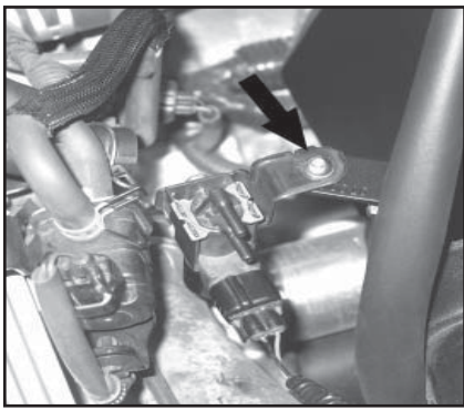
24. Secure the "vacuum switching valve" to the bracket installed onto the heat shield installed in step # 16.
