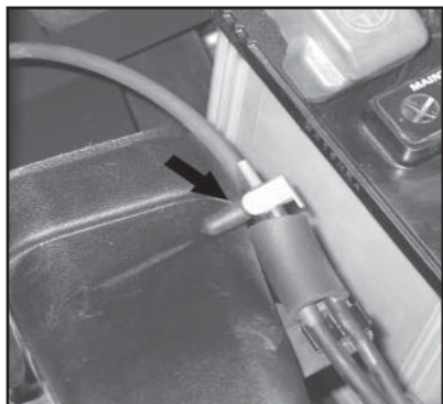
27. Install one vacuum cap plug onto the the factory "T" fitting as shown in the photograph.
