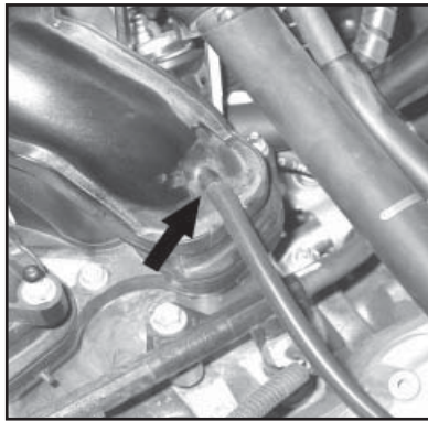
29. Connect the open end of the vacuum line installed in the previous step to the intake manifold plenum connection.
