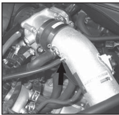
30. Install the supplied vacuum hose to the K&N Intake Tube.
