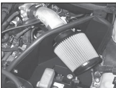
32. Install the K&N Air Filter onto the K&N Intake Tube; secure with the provided hose clamp.
