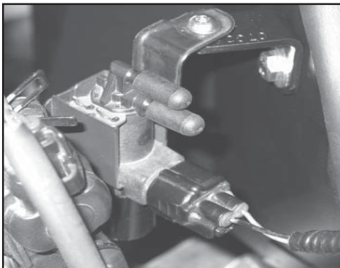
26. Install the two vacuum cap plugs onto the "vacuum switching valve."
