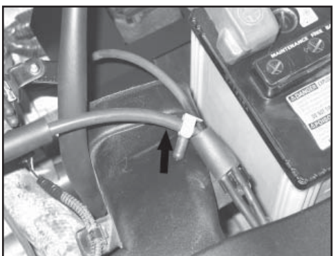
28. Install the supplied vacuum hose onto the factory "T" fitting as shown in the photograph.
