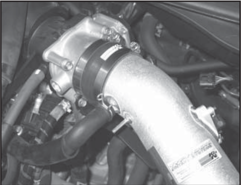
25. Connect the crank case vent hose to the fitting on the K&N Intake Tube; secure with the factory spring clamp.
