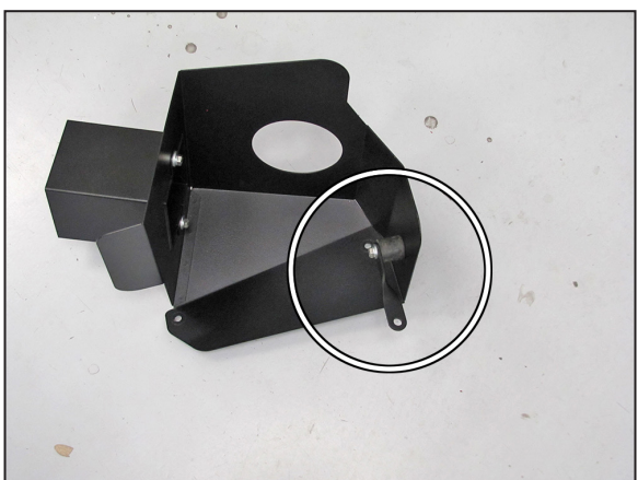
16. Install the bracket assembly onto the heat shield as shown and secure with the provided hardware.
