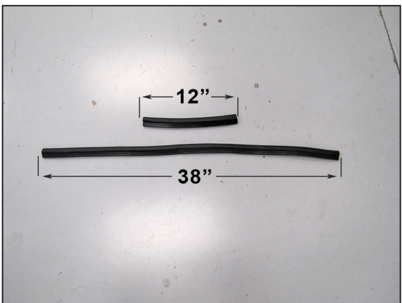
17. Cut the provided edge trim into two sections. One section should be cut to 12" long and the next section should be cut to 38" long.
