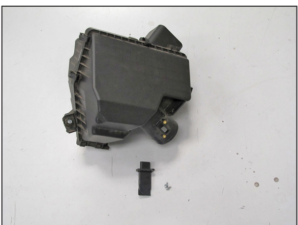
20. Remove the mass air sensor from the factory air box.
