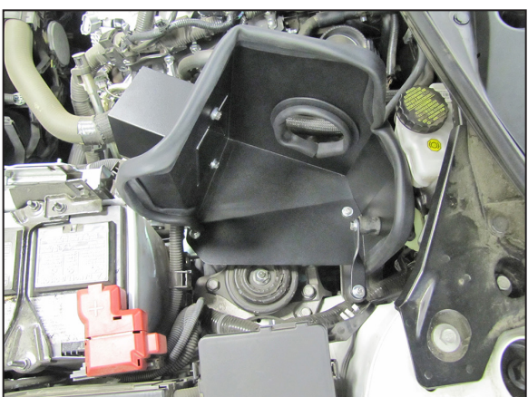
19. Install the heat shield assembly onto the rubber mounted studs and secure with the provided hardware.
