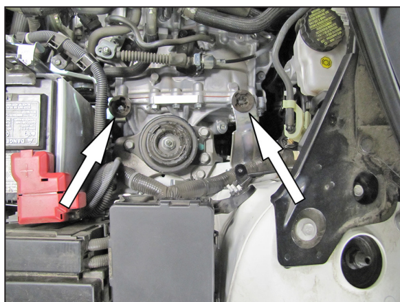
11. Remove the two air box mounting grommets from the mounting brackets shown.
