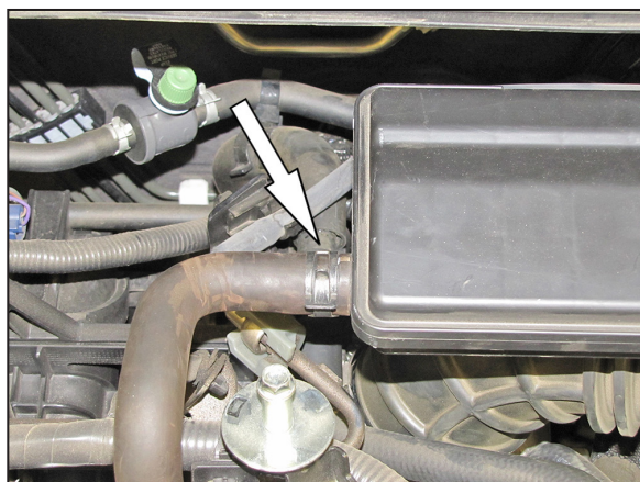
8. Release the spring clamp securing the crank case vent hose to the intake plenum and then disconnect the hose from the plenum.
