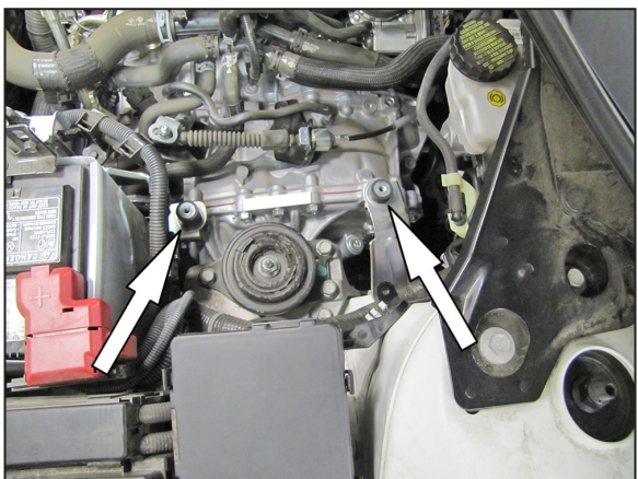
12. Mount the two rubber mounted studs to the air box mounting brackets as shown.
