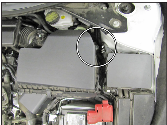
7. Remove the bolt securing the air box to the bracket on the shock tower then lift up the air box to remove it from the vehicle.
