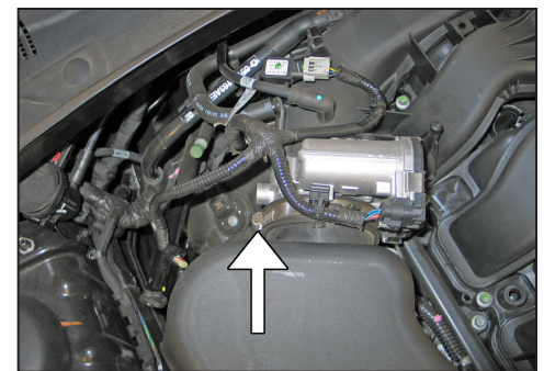
5. Loosen the hose clamp that secures the intake tube to the throttle body.
