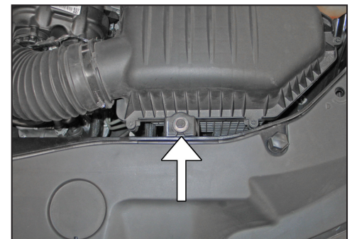
6. Remove the bolt that secures the air filter housing to the core support.
