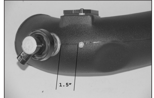
21c. On vehicles equipped with an air temperature sensor, drill a 5/8" hole at the drill point on the K&N intake tube as shown.
