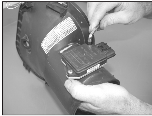
18. On vehicles equipped with a mass air sensor, remove the mass air sensor from the factory air box lid with the provided torx wrench as shown.
