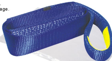
20033 Tree Saver 3' x 6' (30,000lb.)
